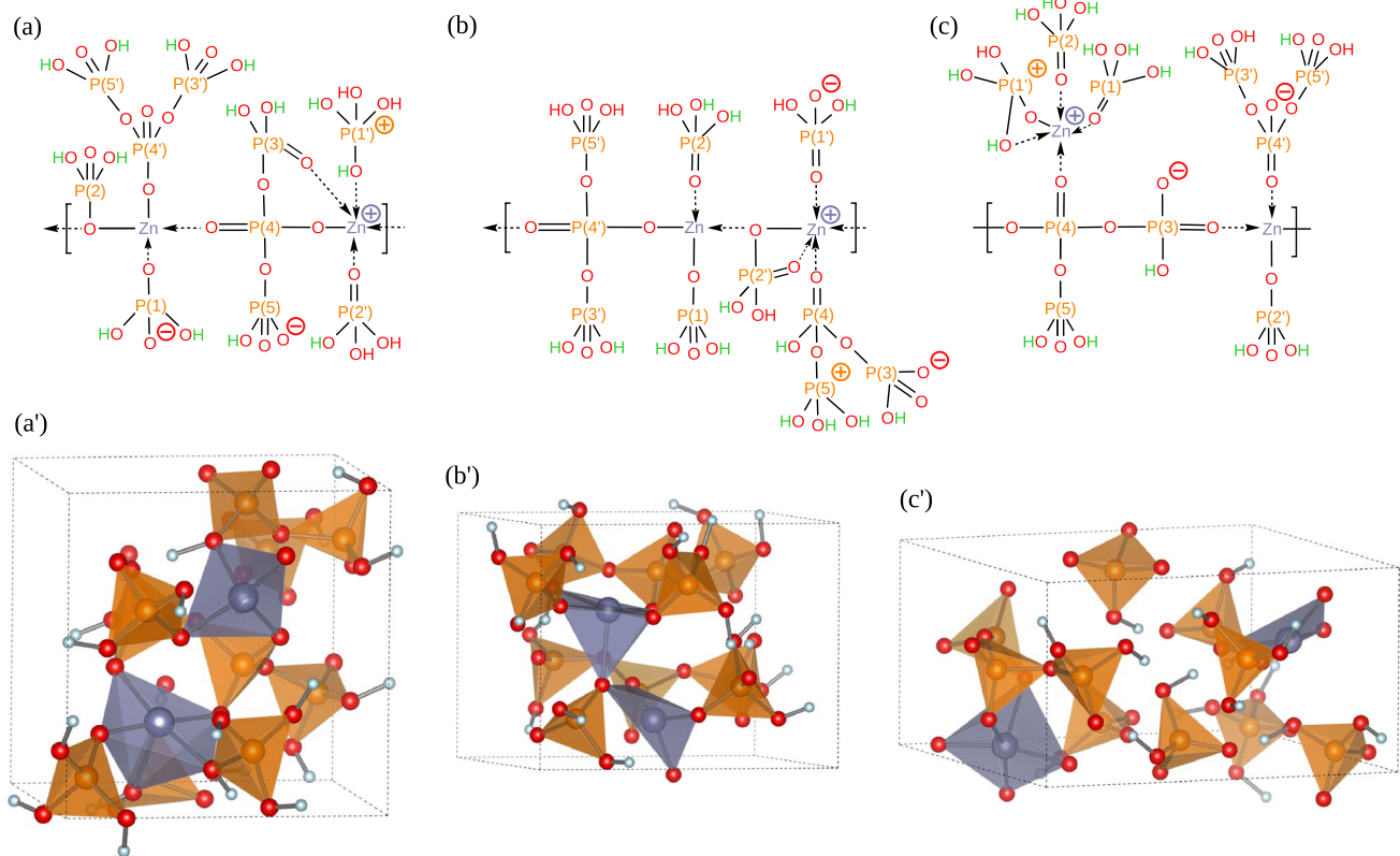
Fig. 2 Lewis (a–c) and three-dimensional (a'–c') structures of the system after decomposition from a isotropic, b uniaxial, and c volume-conserving compressions. Dashed arrows indicate ionic bonds. Zinc, phosphorus and oxygen are presented in gray, orange and red colors, respectively. Formal positive charges are always assigned
