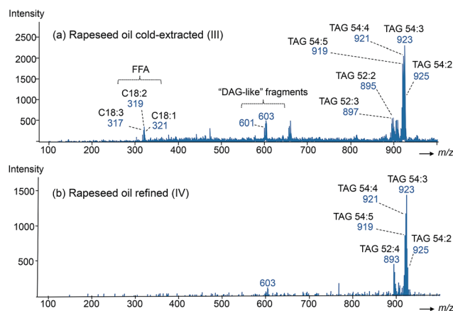
Fig. 5 Pd-NP assisted LDI analyses of commercial rapeseed in positive detection mode using a Pd-NP substrate: (a) cold-extracted oil (III); (b) refined oil (IV). Note: the species' labels and m/z values correspond to [M + K]^+ ions (laser fluence, 45%).
