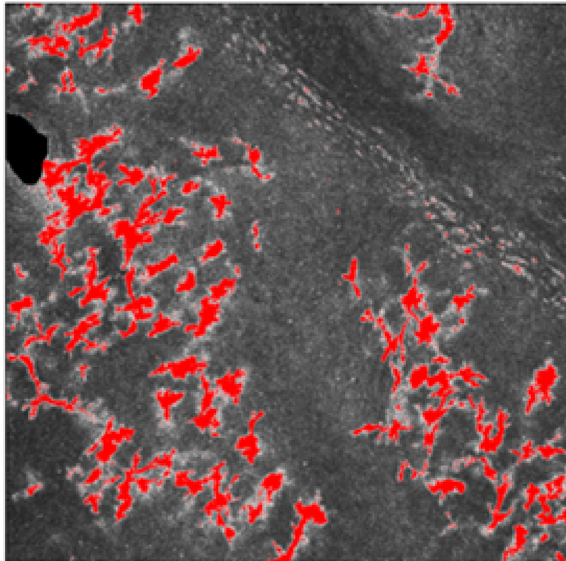
CUD - 254 threshold (9.4%)
